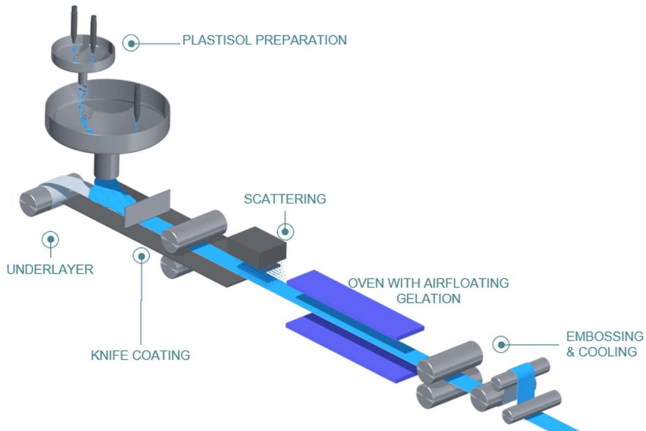
Figure 3: Coating process
